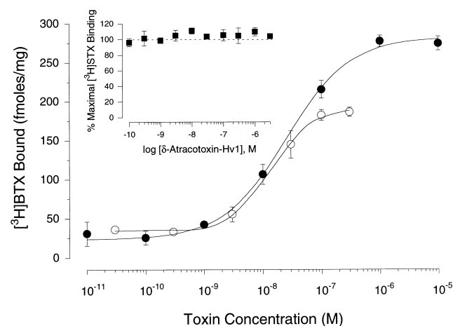
Fig. 3. Effect of \delta -atractoxin-Hv1 on [ 3 H]BTX and [ 3 H]STX binding. Main panel: Enhancement of [ 3 H]BTX by \delta -atractoxin-Hv1 and AaH II. A range of concentrations of AaH II (○) and \delta -atractoxin-Hv1 (●) were incubated with 350 \mu g protein and 15 nM [ 3 H]BTX at 37°C for 50 min. Data are presented as fmol of [ 3 H]BTX bound per mg of synaptosomal protein following correction for non-specific binding determined in the presence of 300 \mu M veratridine. Values represent the mean \pm S.E. of 4 experiments. Inset: No alteration in [ 3 H]STX binding by \delta -atractoxin-Hv1. A range of concentrations of \delta -atractoxin-Hv1 were incubated with rat brain synaptosomes in the presence of 2 nM [ 3 H]STX at 37°C for 30 min. Data are presented as the percentage of maximal [ 3 H]STX binding following correction for non-specific binding determined in the presence of 1 \mu M TTX. The dashed line represents [ 3 H]STX binding in the absence of \delta -atractoxin-Hv1. Values represent the mean \pm S.E. of 5 experiments.
